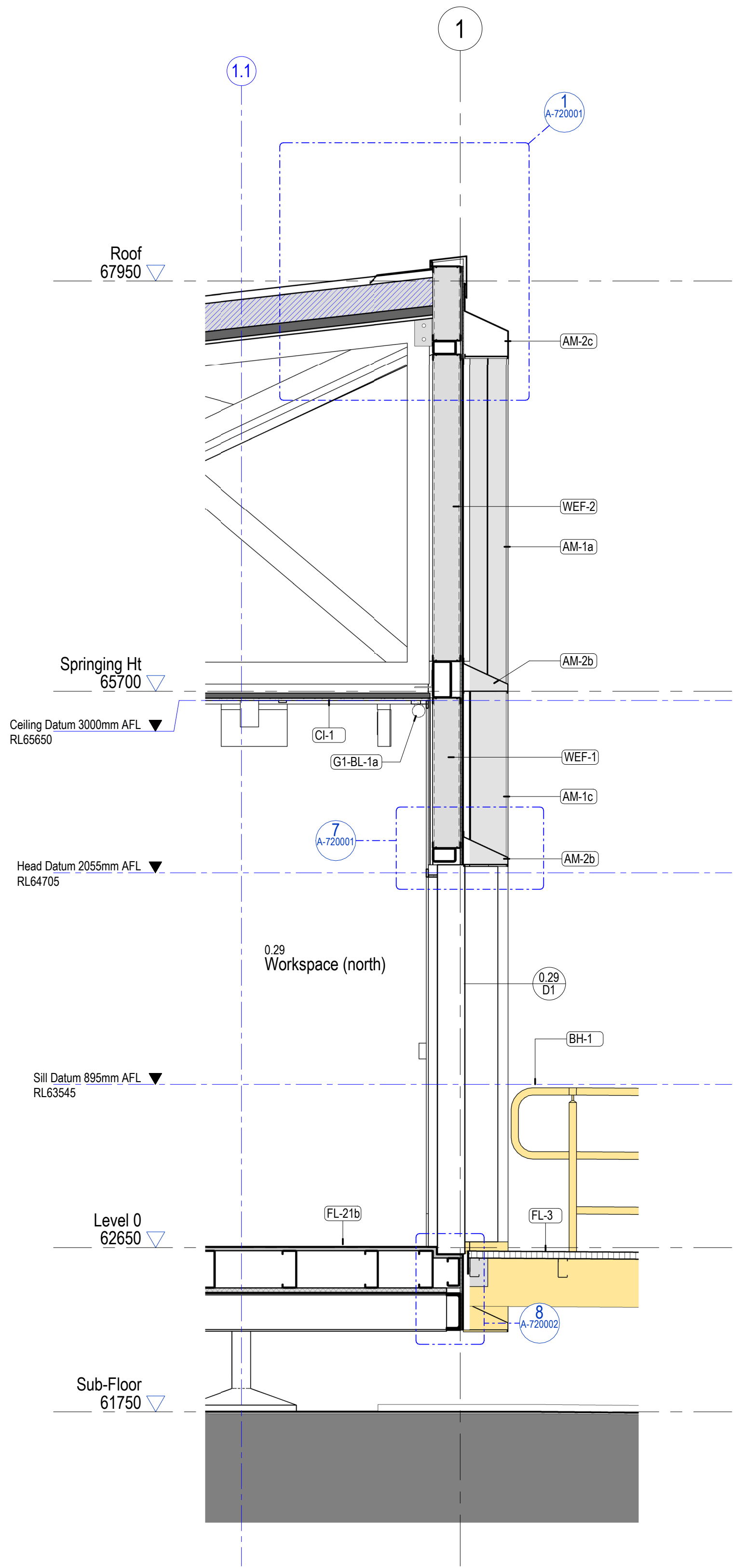
1 North Entry Facade Section 1 : 20 Workplace North
