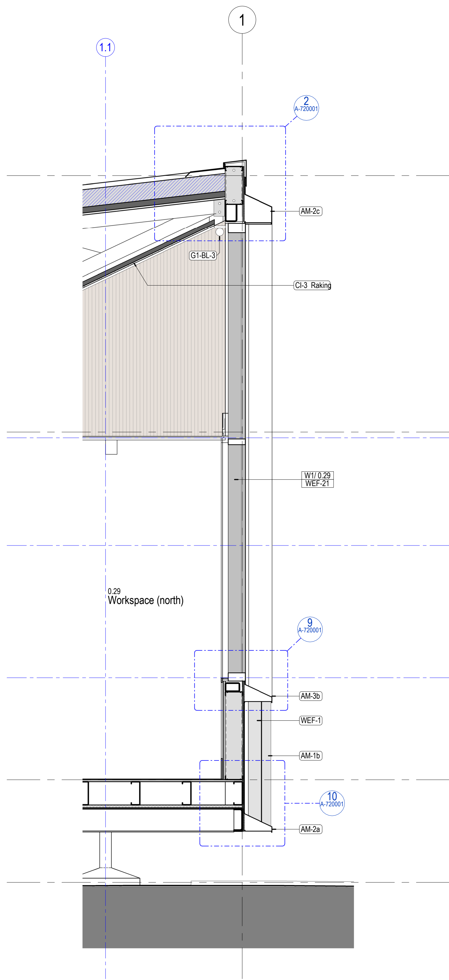
2 North Full Height Window Section 1 : 20 Workplace North
